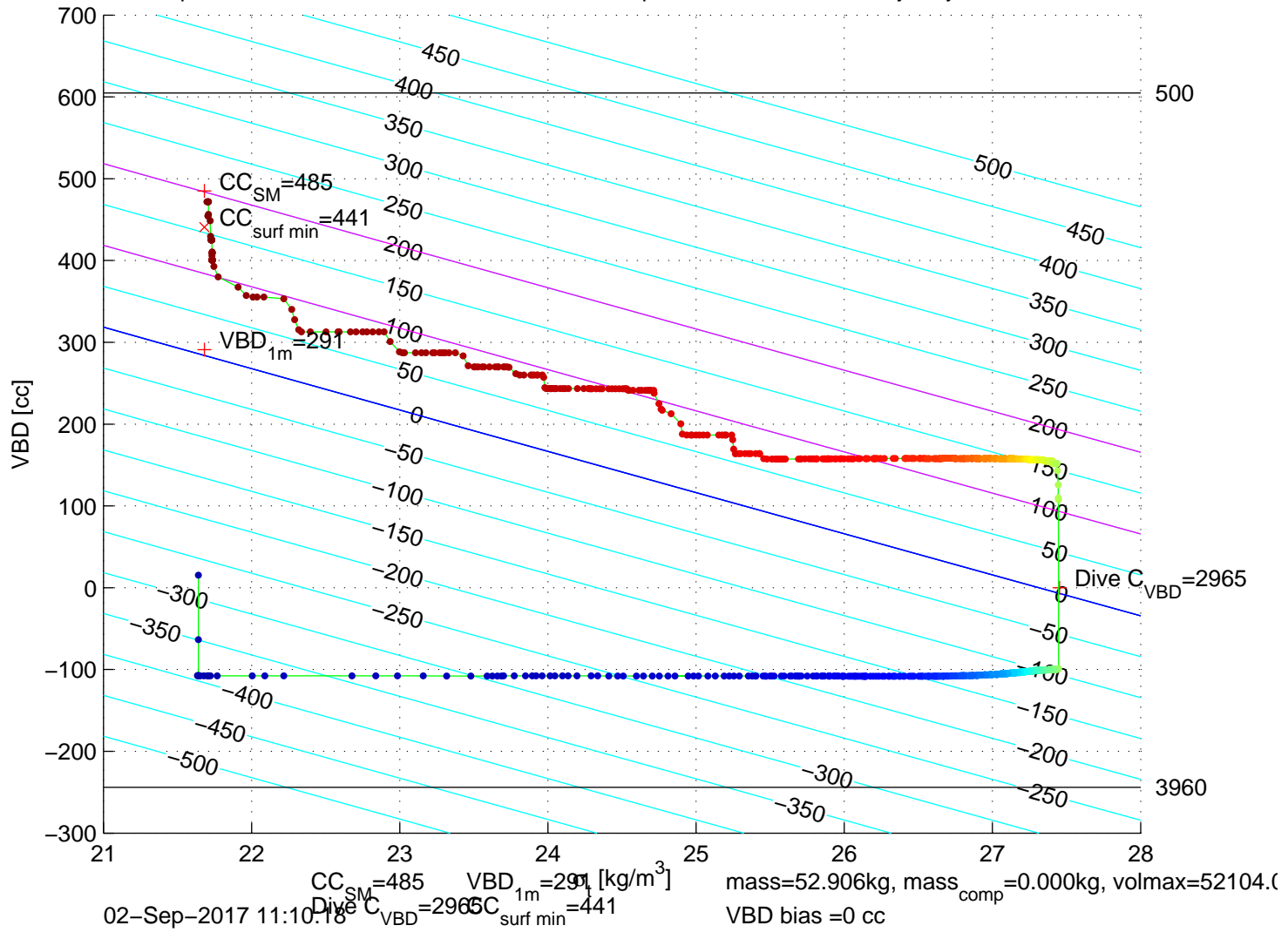
p6100323: SG610 Mission 7 Jul 2017 02-Sep-2017 10:39:17Z – buoyancy contoured
