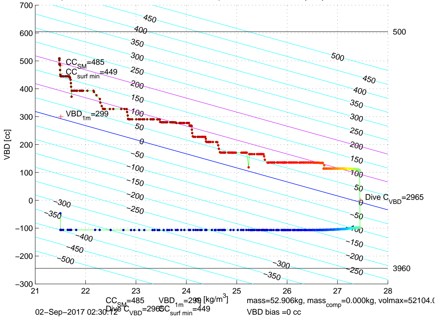
p6100321: SG610 Mission 7 Jul 2017 02-Sep-2017 01:48:13Z – buoyancy contoured
