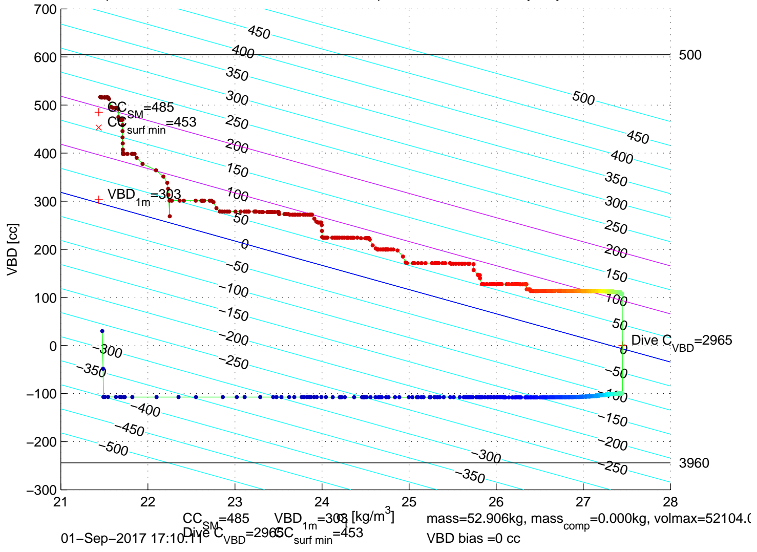
p6100319: SG610 Mission 7 Jul 2017 01-Sep-2017 16:22:17Z – buoyancy contoured
