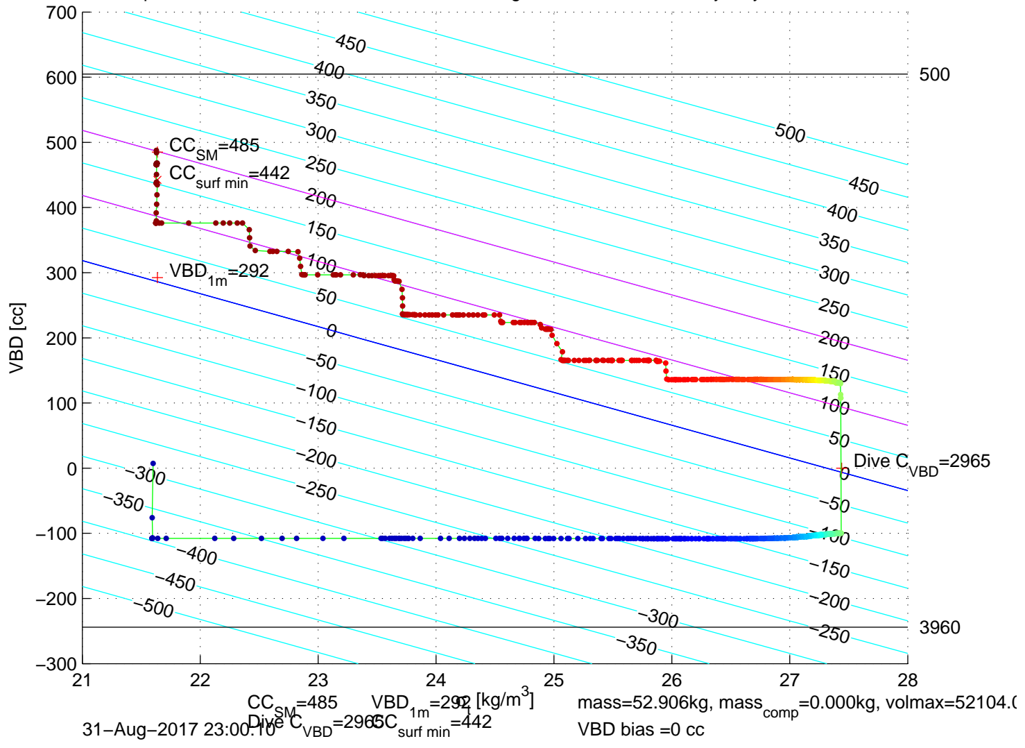
p6100315: SG610 Mission 7 Jul 2017 31-Aug-2017 22:29:09Z – buoyancy contoured
