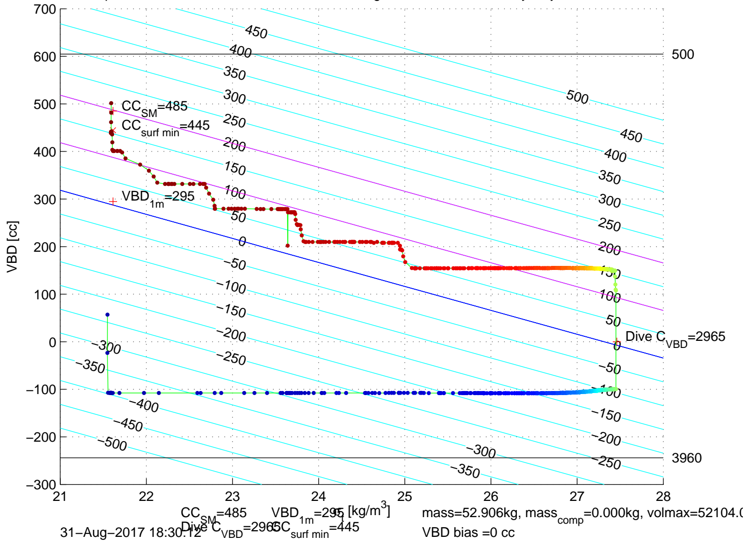
p6100314: SG610 Mission 7 Jul 2017 31-Aug-2017 18:05:16Z – buoyancy contoured
