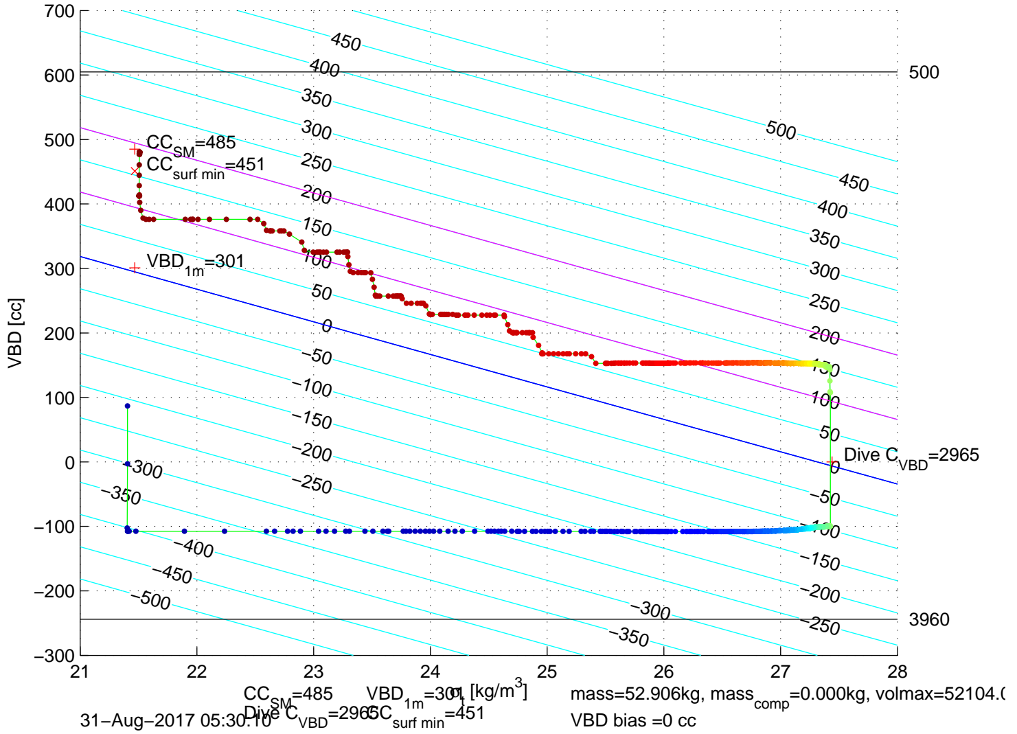
p6100311: SG610 Mission 7 Jul 2017 31-Aug-2017 05:05:43Z – buoyancy contoured
