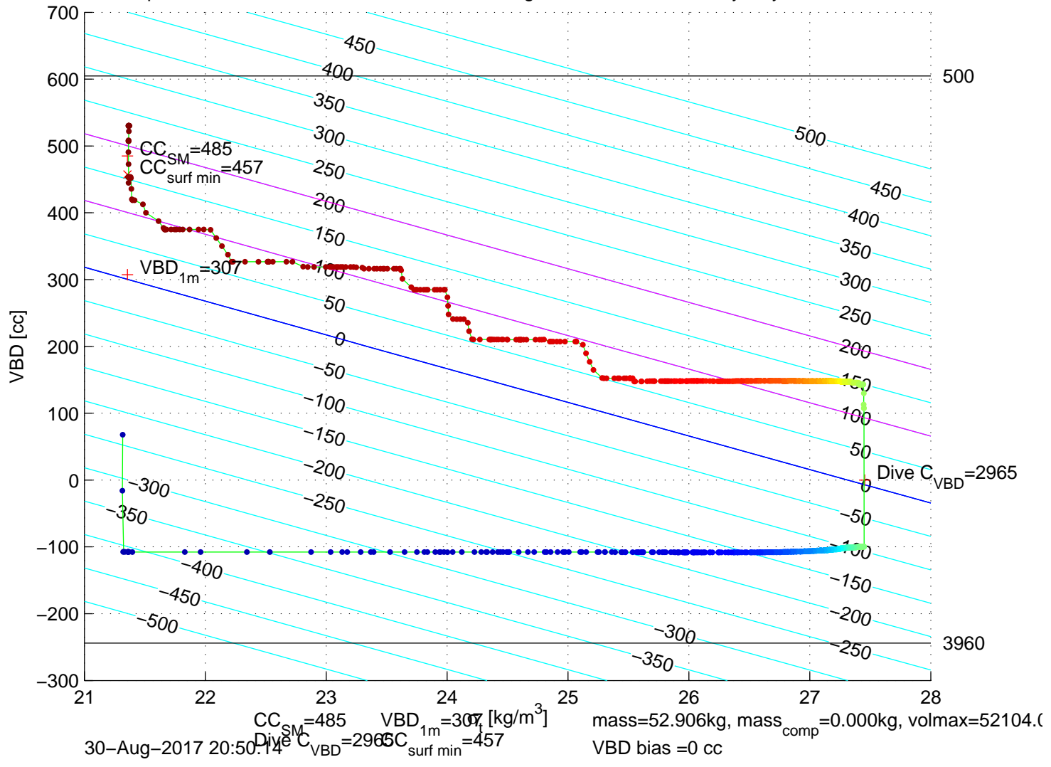
p6100309: SG610 Mission 7 Jul 2017 30-Aug-2017 20:19:57Z – buoyancy contoured
