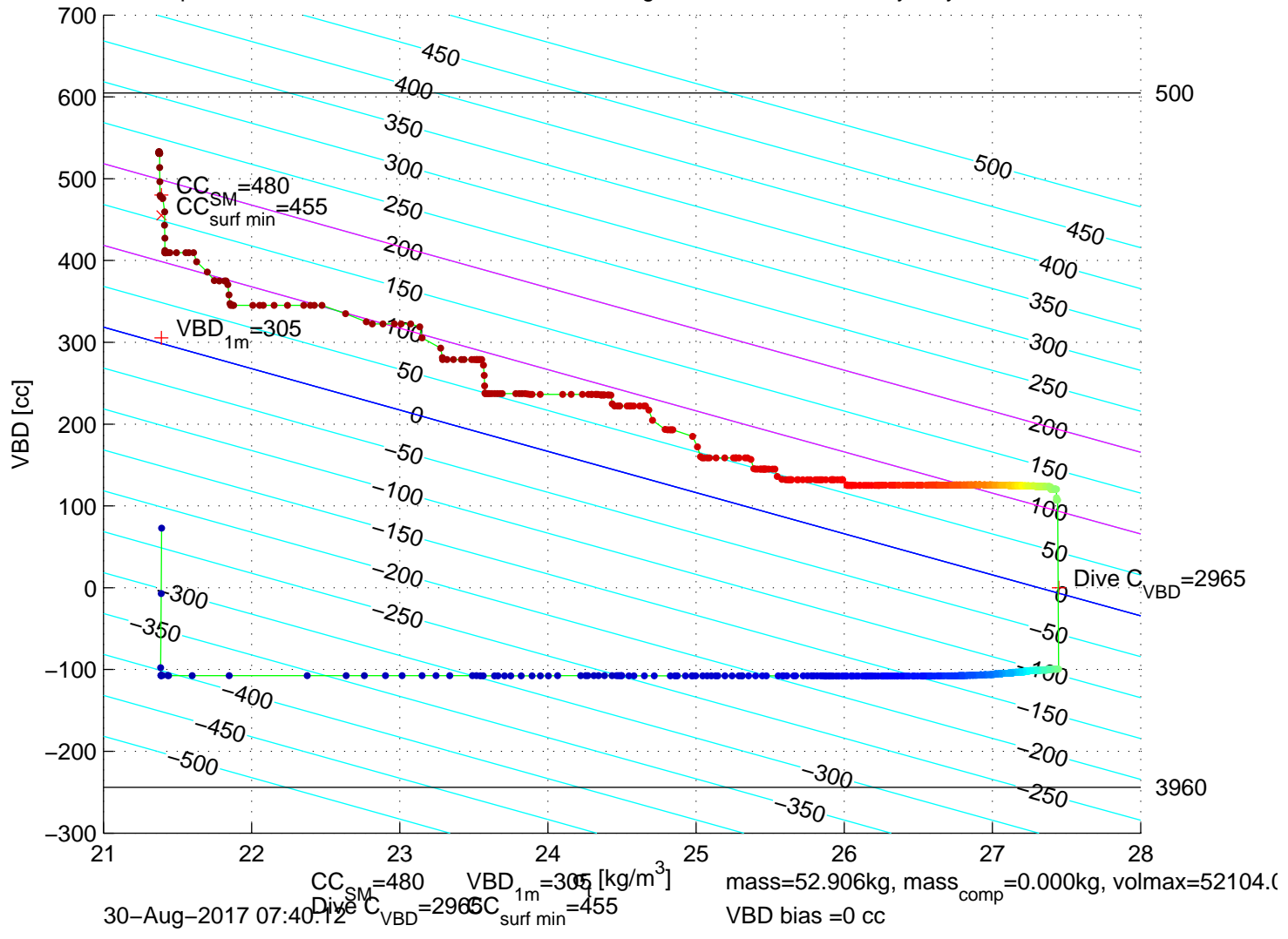
p6100306: SG610 Mission 7 Jul 2017 30-Aug-2017 06:57:20Z – buoyancy contoured
