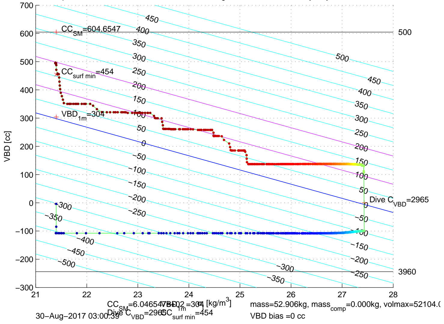
p6100305: SG610 Mission 7 Jul 2017 30-Aug-2017 02:29:23Z – buoyancy contoured
