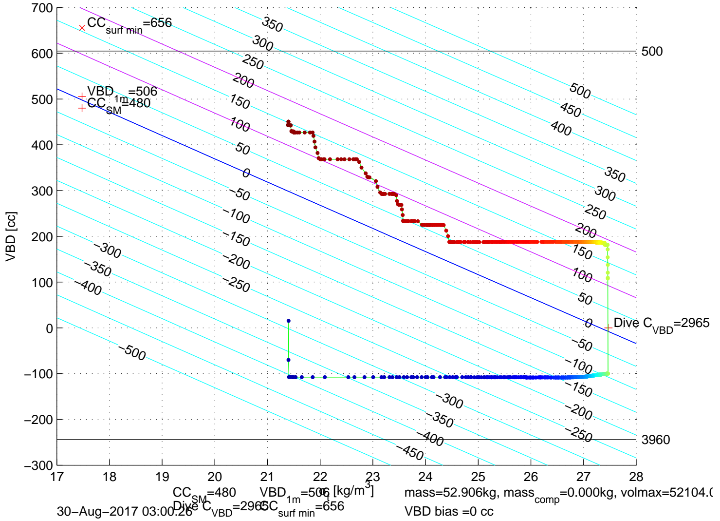
p6100304: SG610 Mission 7 Jul 2017 29–Aug–2017 22:21:29Z – buoyancy contoured
