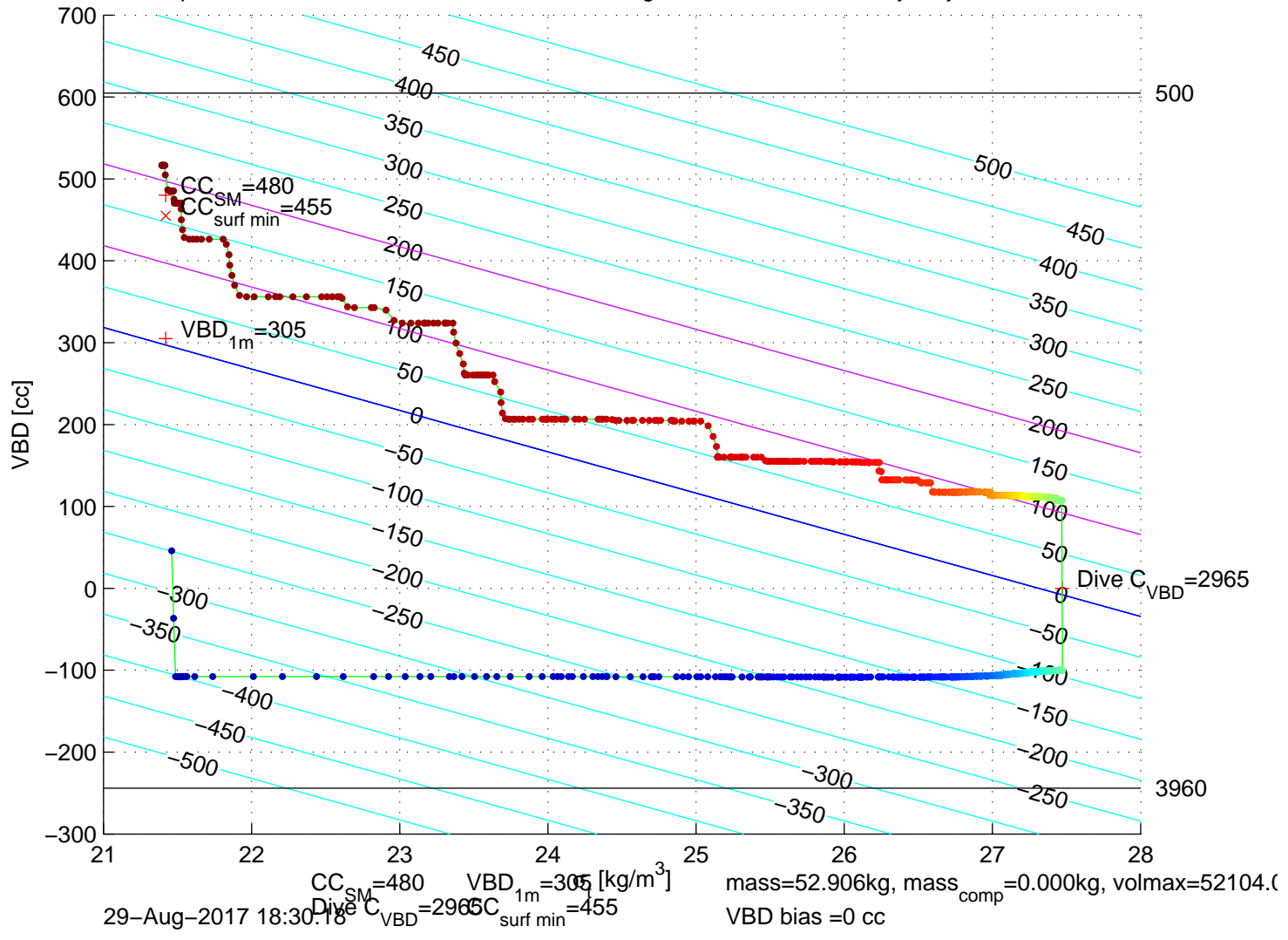
p6100303: SG610 Mission 7 Jul 2017 29-Aug-2017 17:42:44Z – buoyancy contoured
