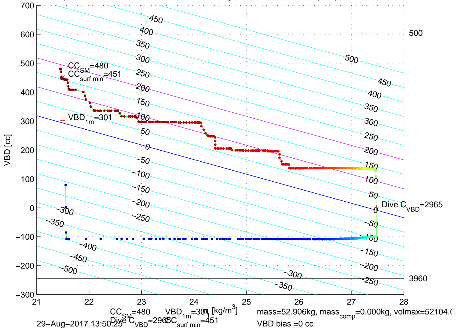
p6100302: SG610 Mission 7 Jul 2017 29-Aug-2017 13:09:55Z – buoyancy contoured
