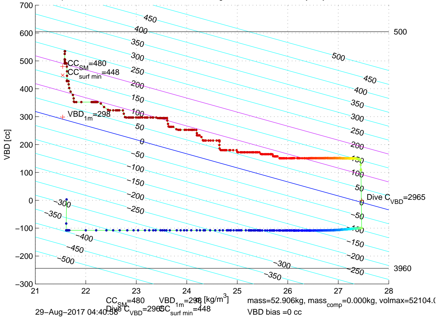
p6100300: SG610 Mission 7 Jul 2017 29-Aug-2017 04:01:19Z – buoyancy contoured
