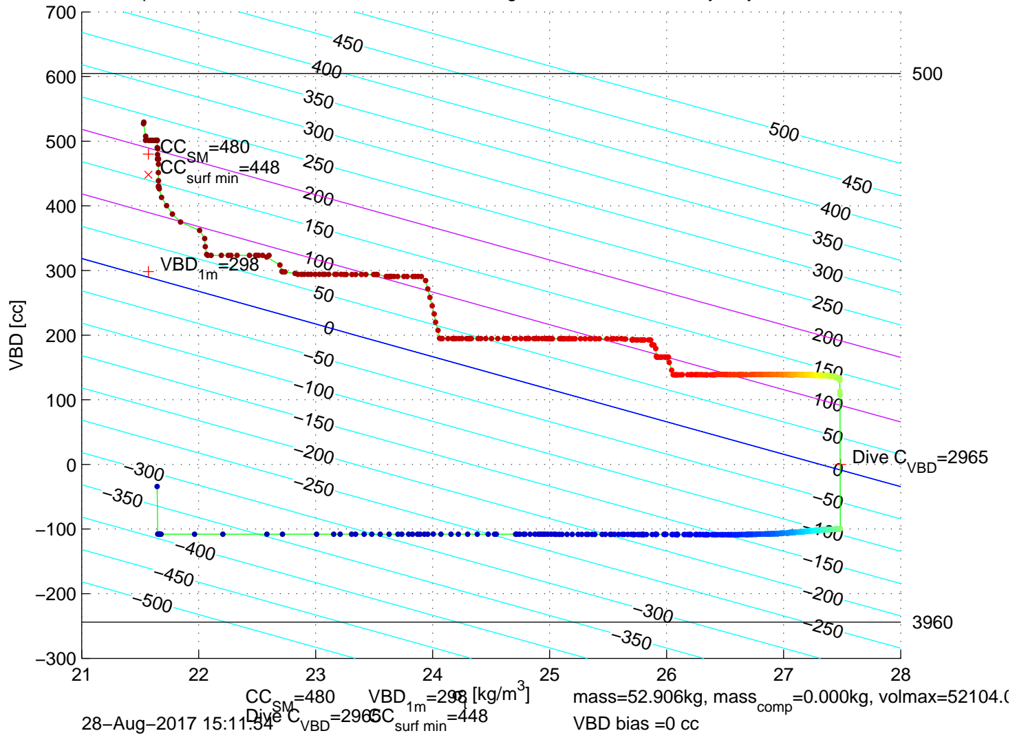
p6100297: SG610 Mission 7 Jul 2017 28-Aug-2017 14:29:54Z – buoyancy contoured
