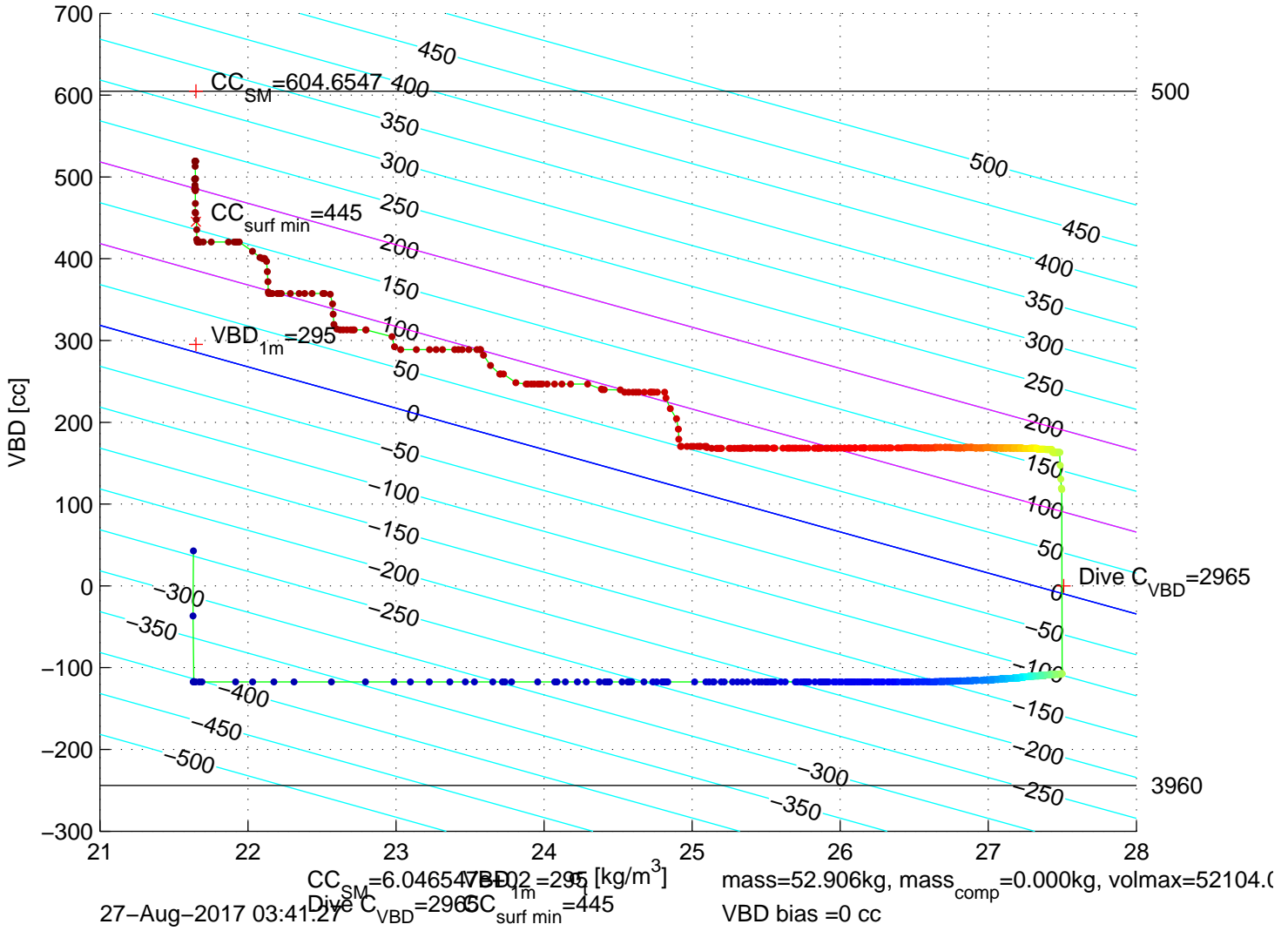
p6100289: SG610 Mission 7 Jul 2017 27-Aug-2017 03:06:07Z – buoyancy contoured
