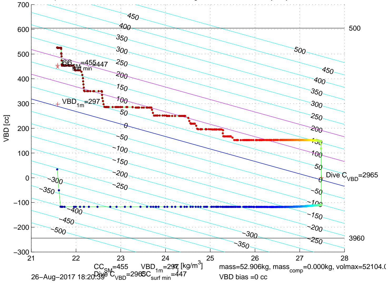
p6100287: SG610 Mission 7 Jul 2017 26-Aug-2017 17:49:45Z – buoyancy contoured
