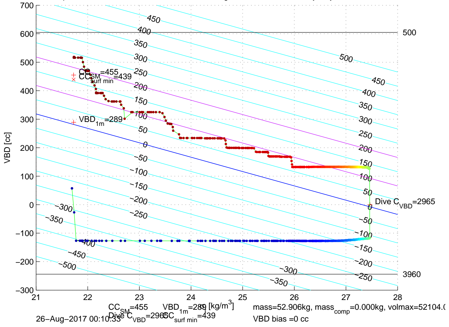
p6100283: SG610 Mission 7 Jul 2017 25-Aug-2017 23:25:12Z – buoyancy contoured
