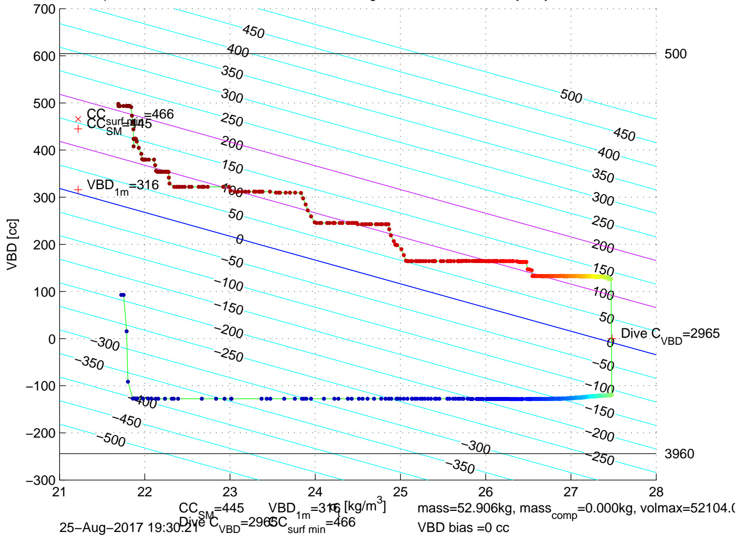
p6100282: SG610 Mission 7 Jul 2017 25-Aug-2017 18:42:32Z – buoyancy contoured
