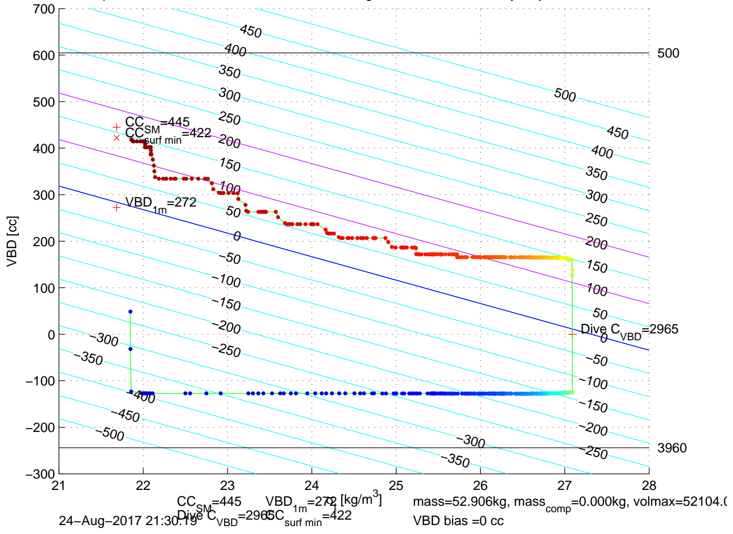
p6100275: SG610 Mission 7 Jul 2017 24-Aug-2017 22:51:04Z – buoyancy contoured
