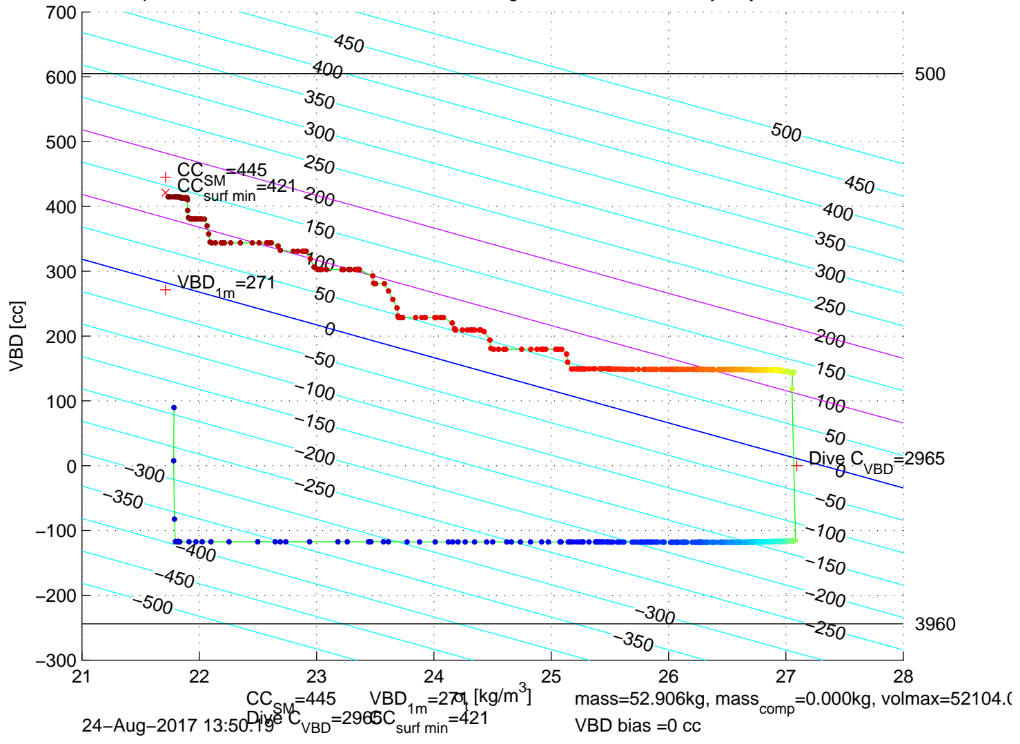
p6100272: SG610 Mission 7 Jul 2017 24-Aug-2017 15:13:42Z – buoyancy contoured
