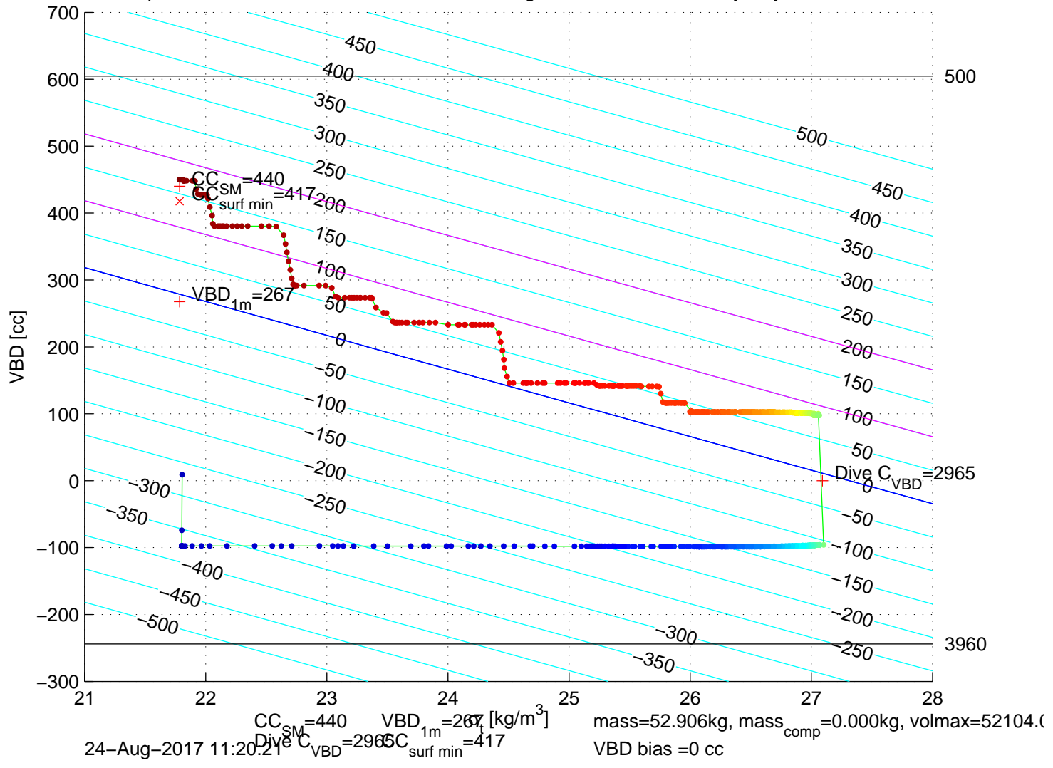
p6100271: SG610 Mission 7 Jul 2017 24-Aug-2017 12:28:35Z – buoyancy contoured
