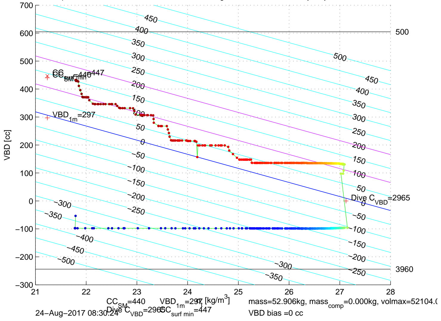
p6100270: SG610 Mission 7 Jul 2017 24-Aug-2017 09:50:57Z – buoyancy contoured
