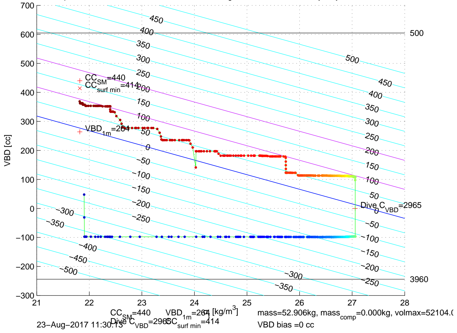
p6100262: SG610 Mission 7 Jul 2017 23-Aug-2017 12:47:55Z – buoyancy contoured
