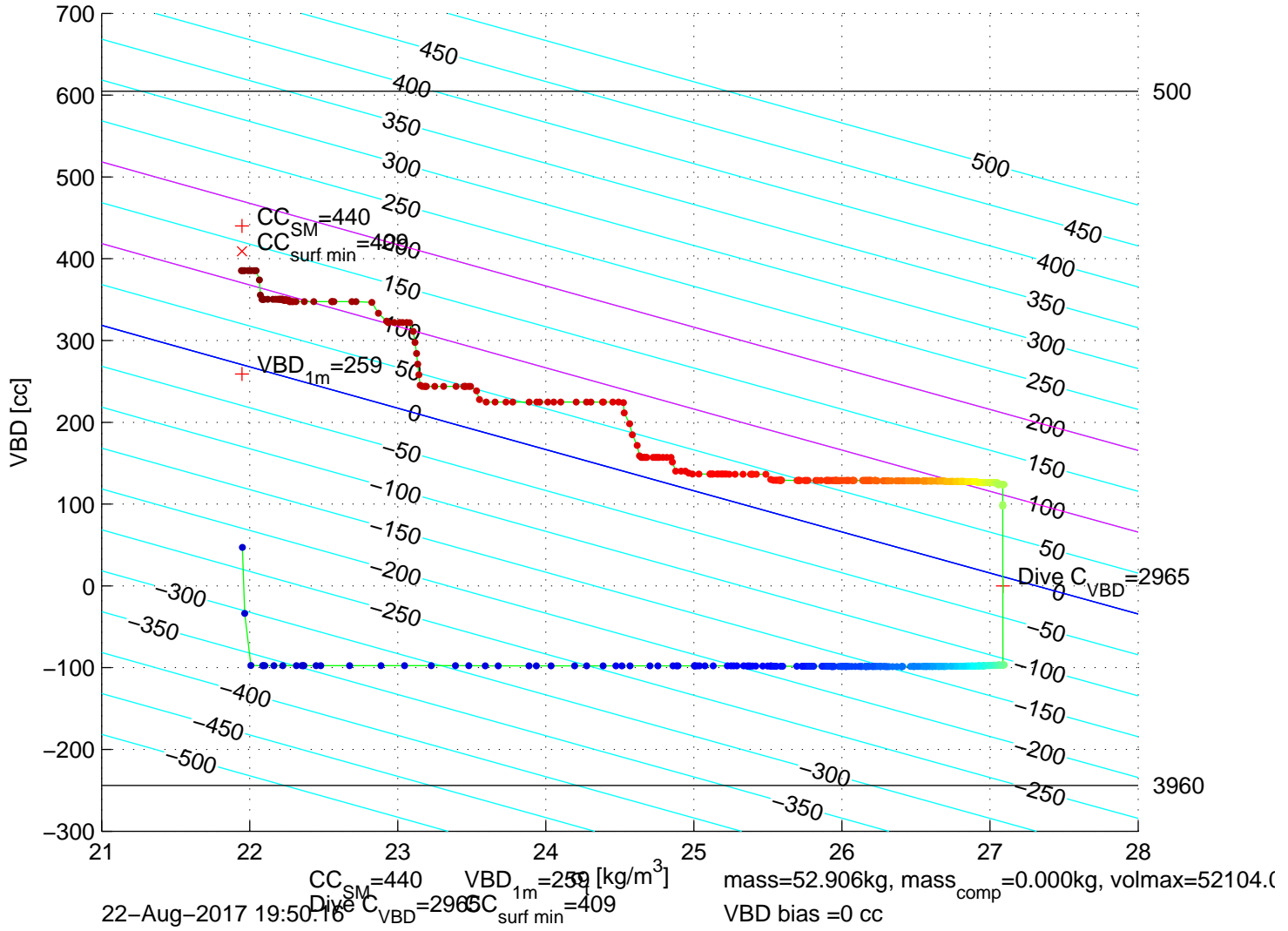
p6100256: SG610 Mission 7 Jul 2017 22-Aug-2017 21:05:34Z – buoyancy contoured
