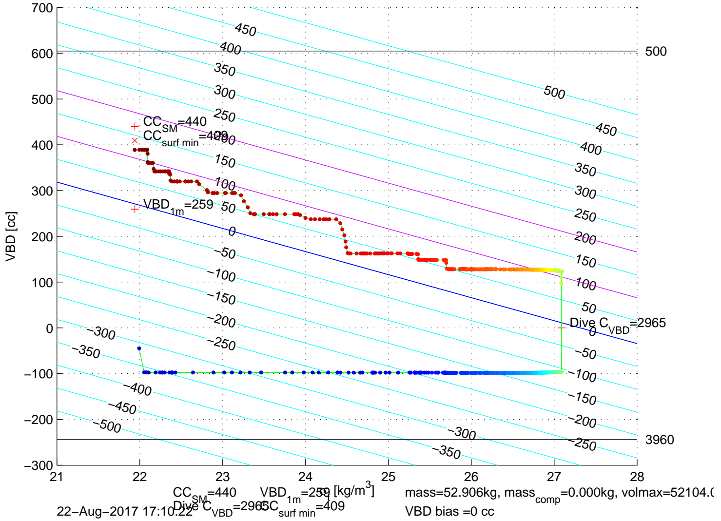
p6100255: SG610 Mission 7 Jul 2017 22-Aug-2017 18:30:39Z – buoyancy contoured
