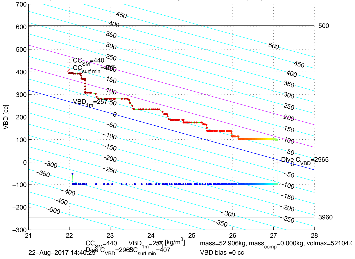
p6100254: SG610 Mission 7 Jul 2017 22-Aug-2017 15:53:04Z – buoyancy contoured
