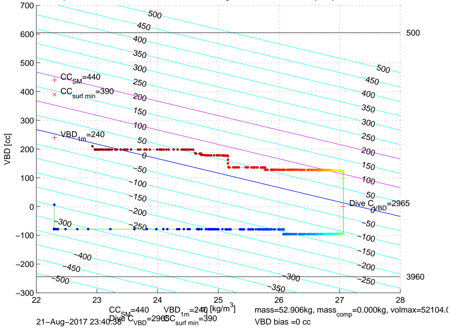
p6100248: SG610 Mission 7 Jul 2017 22-Aug-2017 01:05:35Z – buoyancy contoured
