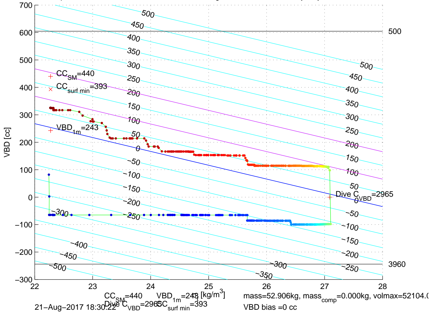
p6100246: SG610 Mission 7 Jul 2017 21-Aug-2017 20:06:23Z – buoyancy contoured
