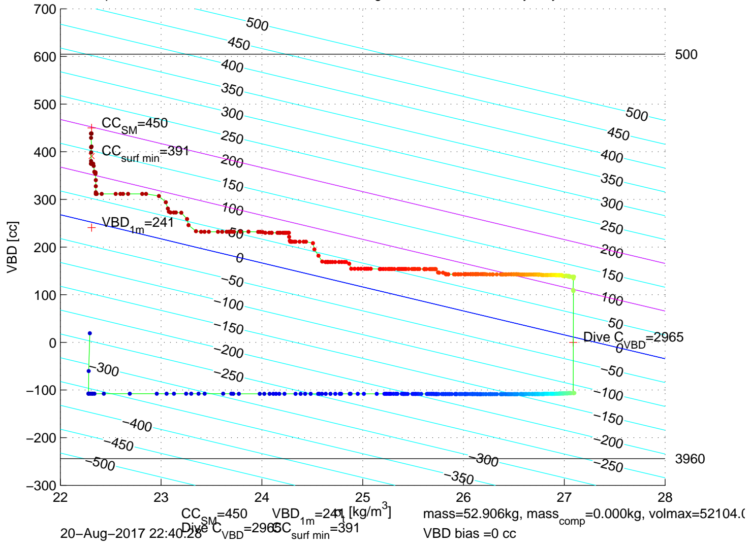
p6100238: SG610 Mission 7 Jul 2017 21-Aug-2017 00:08:06Z – buoyancy contoured
