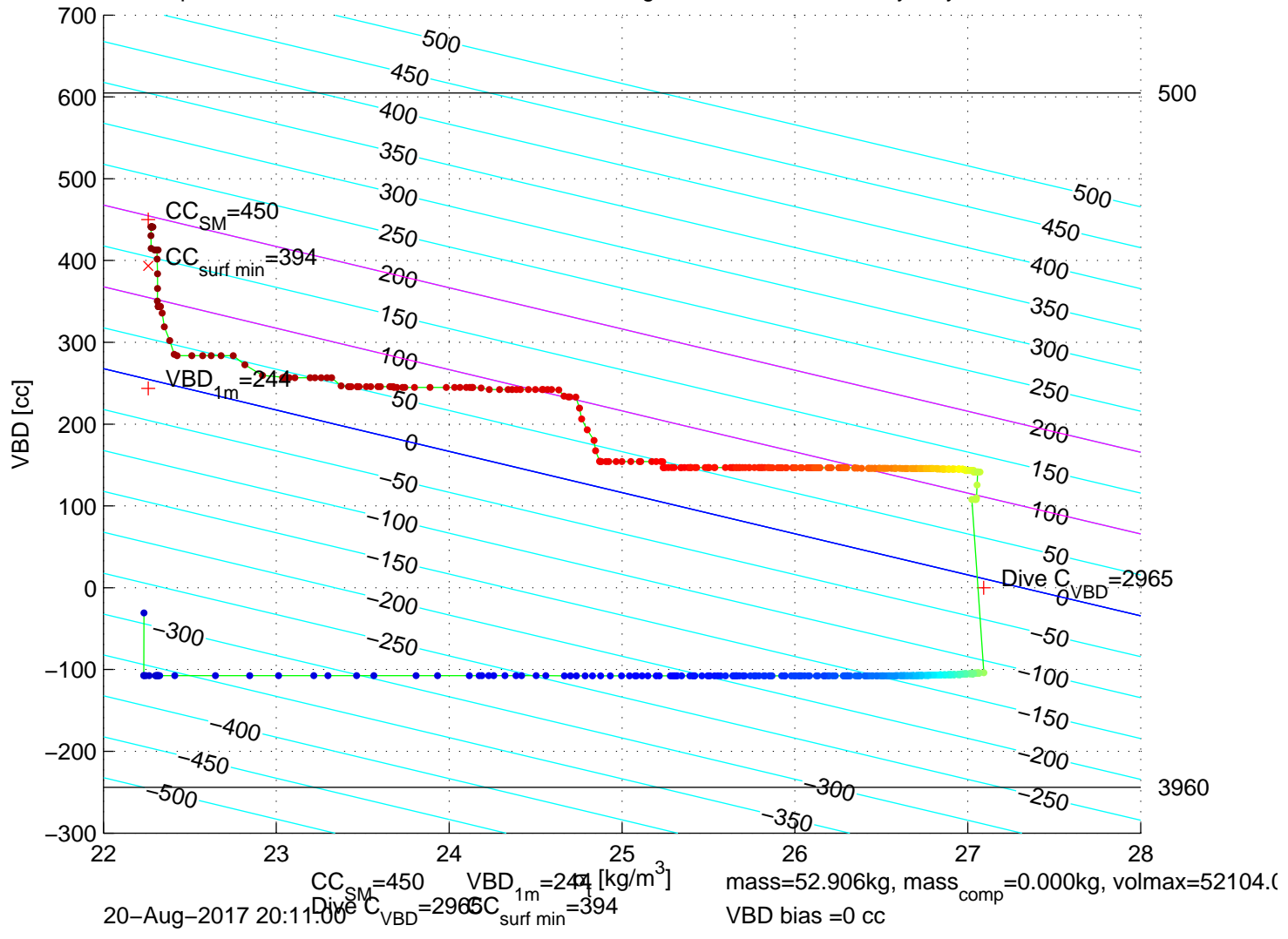
p6100237: SG610 Mission 7 Jul 2017 20–Aug–2017 21:33:50Z – buoyancy contoured
