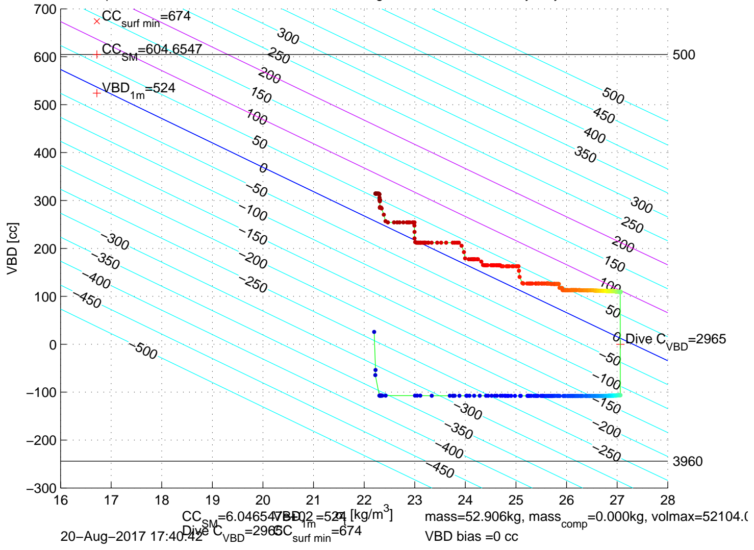
p6100236: SG610 Mission 7 Jul 2017 20-Aug-2017 19:09:35Z – buoyancy contoured
