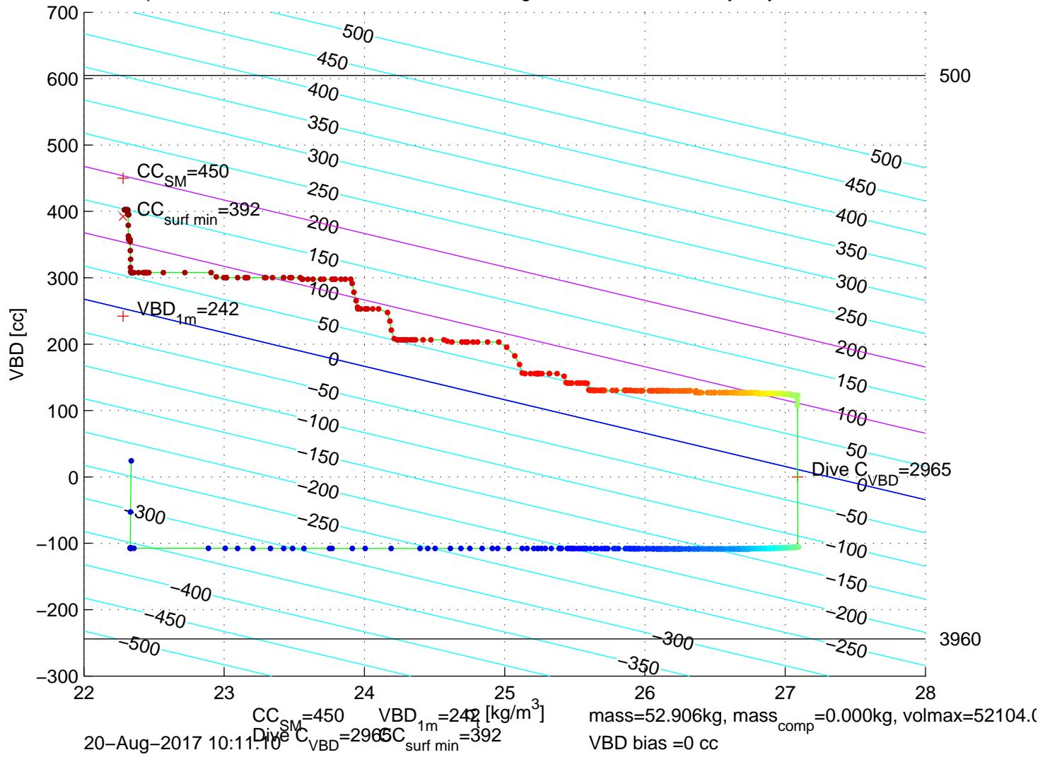
p6100233: SG610 Mission 7 Jul 2017 20-Aug-2017 11:28:37Z – buoyancy contoured
