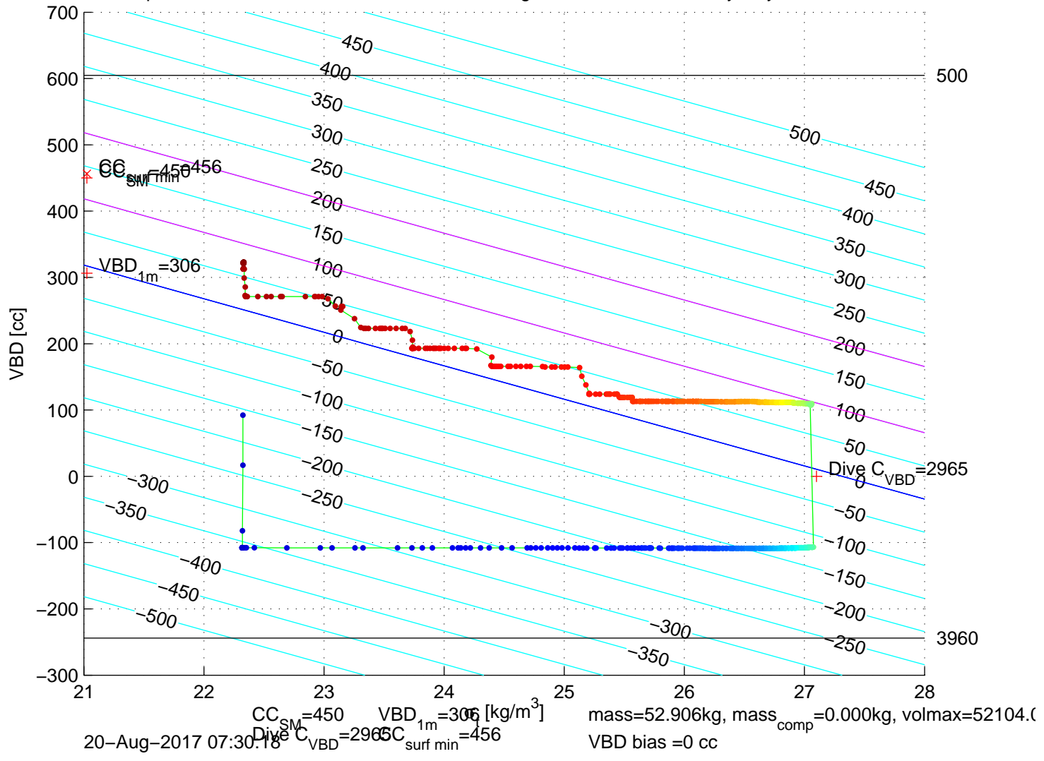
p6100232: SG610 Mission 7 Jul 2017 20-Aug-2017 09:07:03Z – buoyancy contoured
