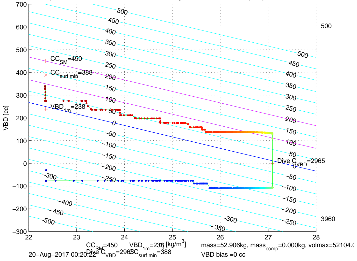
p6100229: SG610 Mission 7 Jul 2017 20-Aug-2017 01:42:24Z - buoyancy contoured
