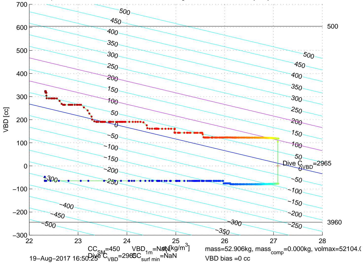
p6100226: SG610 Mission 7 Jul 2017 19–Aug–2017 18:07:59Z – buoyancy contoured
