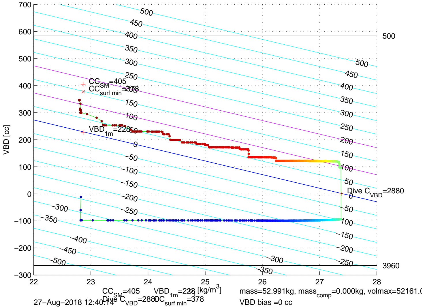
p6100223: SG610 Mission 8 Jul 2018 27-Aug-2018 12:02:22Z – buoyancy contoured
