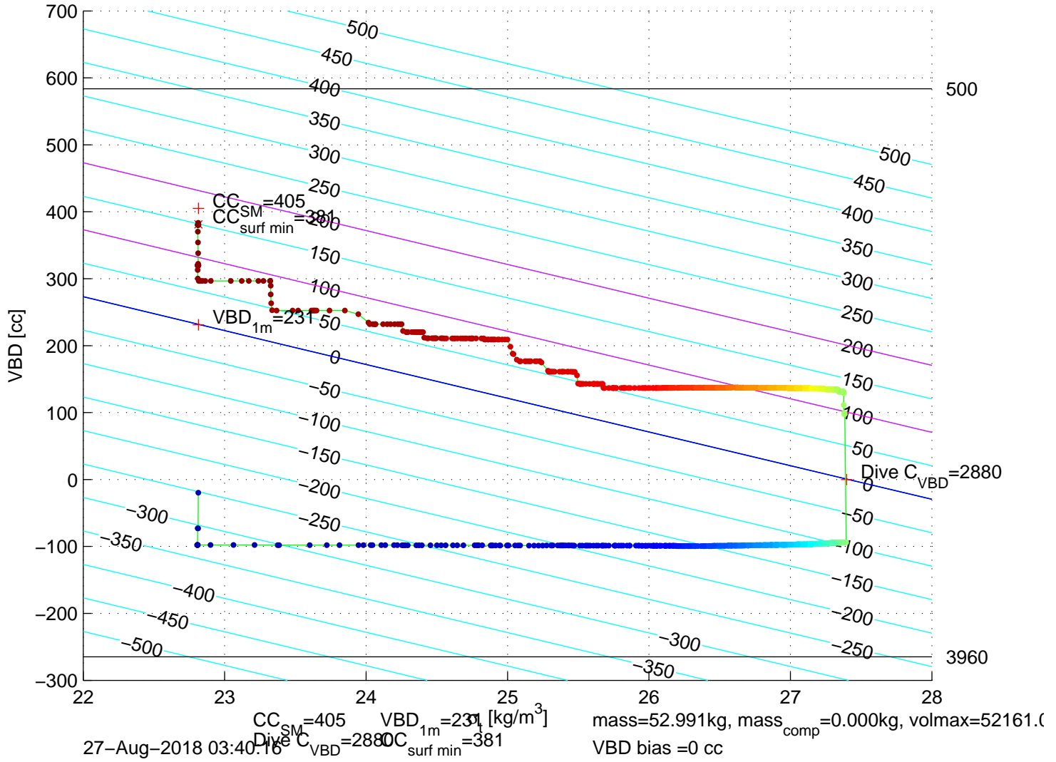
p6100221: SG610 Mission 8 Jul 2018 27-Aug-2018 02:58:17Z – buoyancy contoured
