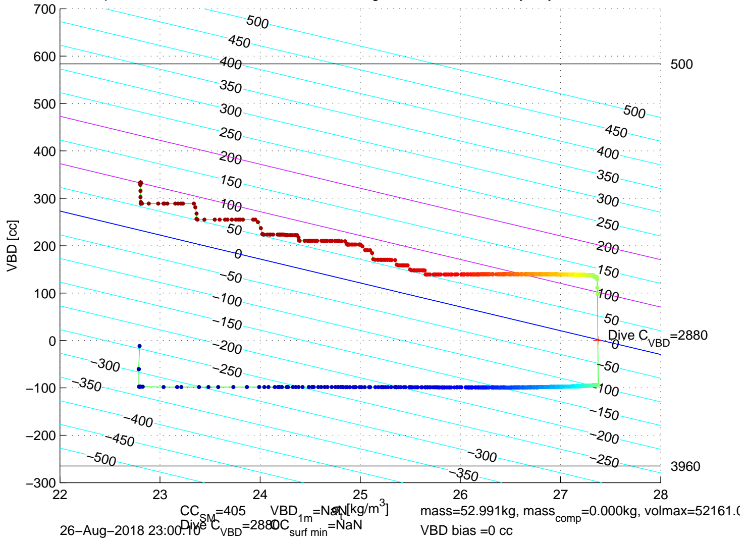
p6100220: SG610 Mission 8 Jul 2018 26-Aug-2018 22:31:49Z – buoyancy contoured
