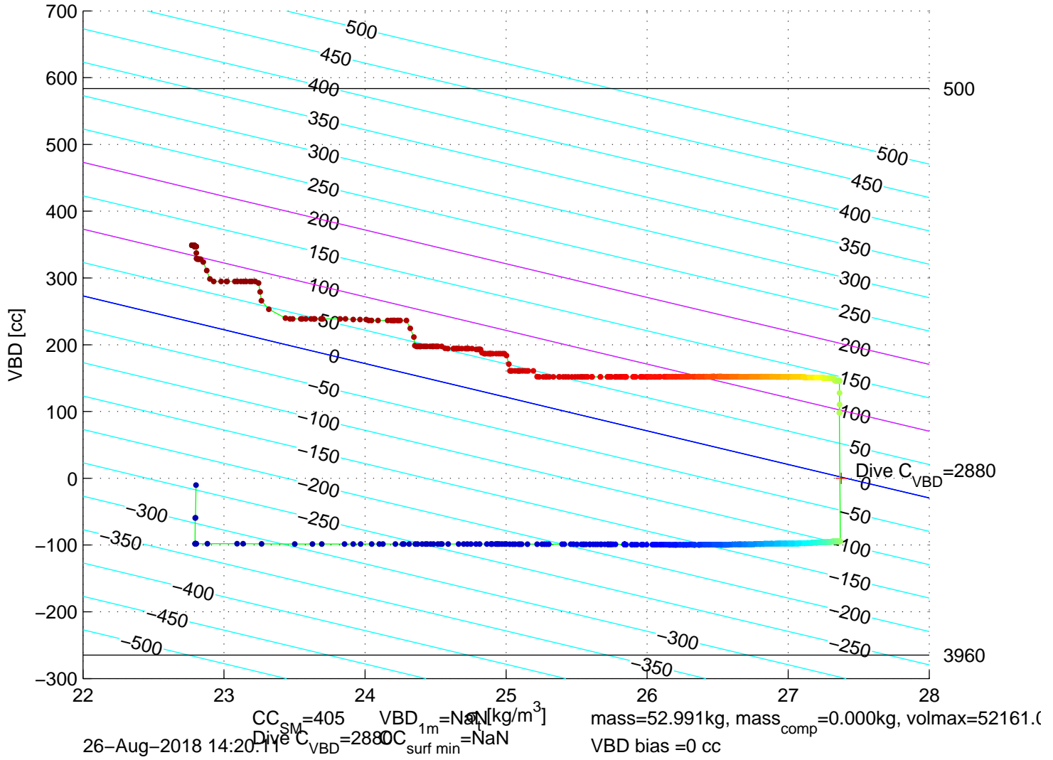
p6100218: SG610 Mission 8 Jul 2018 26-Aug-2018 13:53:29Z – buoyancy contoured
