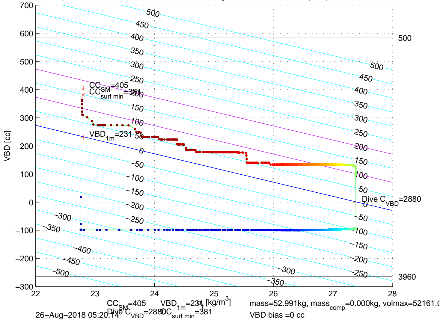
p6100216: SG610 Mission 8 Jul 2018 26-Aug-2018 04:39:55Z – buoyancy contoured
