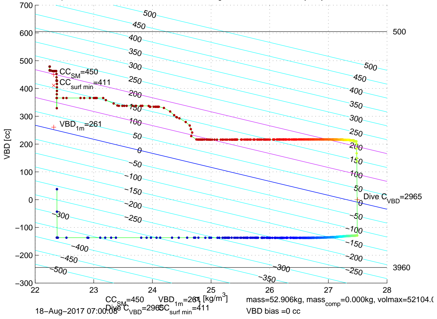
p6100214: SG610 Mission 7 Jul 2017 18-Aug-2017 06:48:35Z – buoyancy contoured
