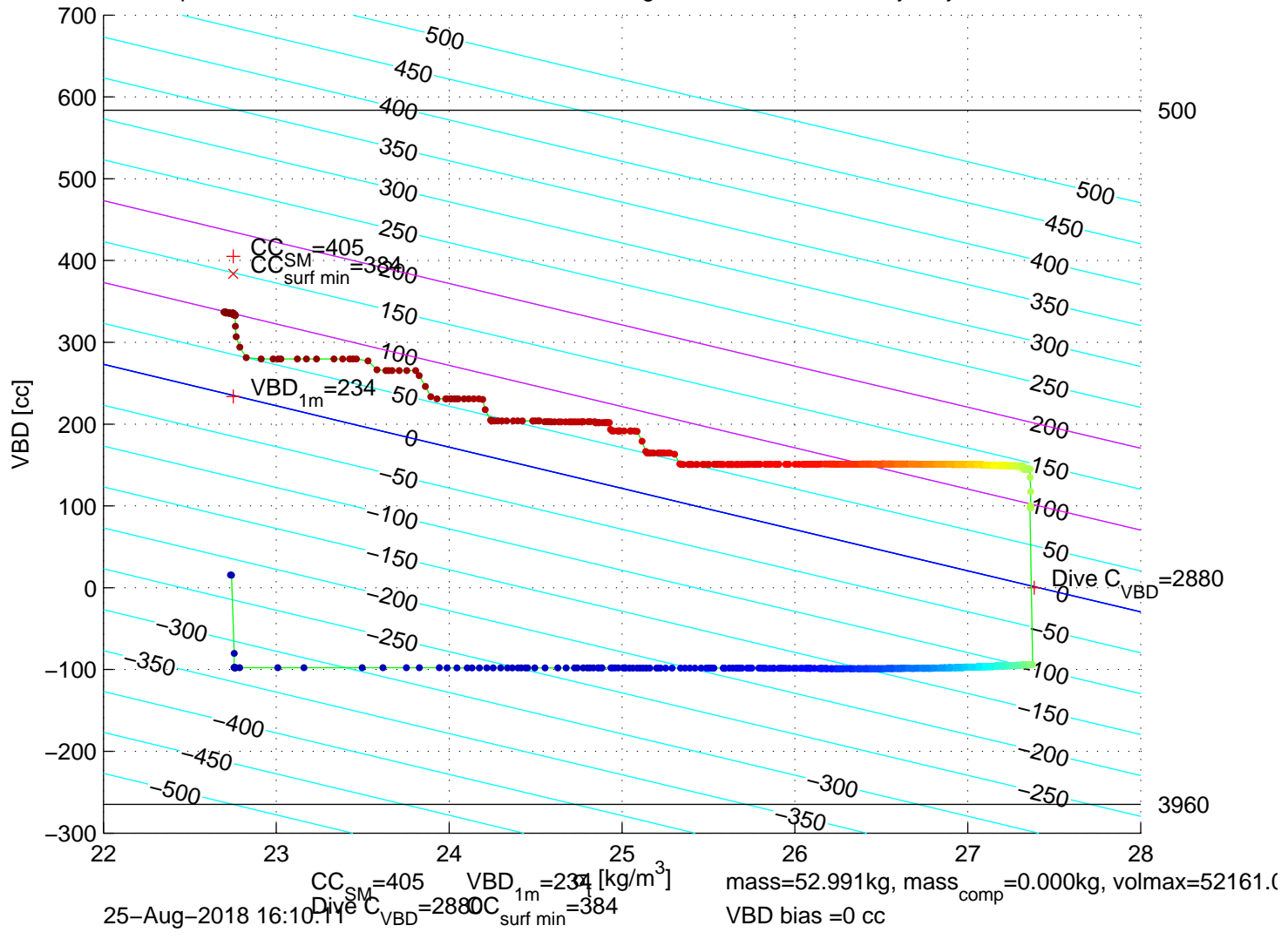
p6100213: SG610 Mission 8 Jul 2018 25-Aug-2018 15:43:41Z – buoyancy contoured
