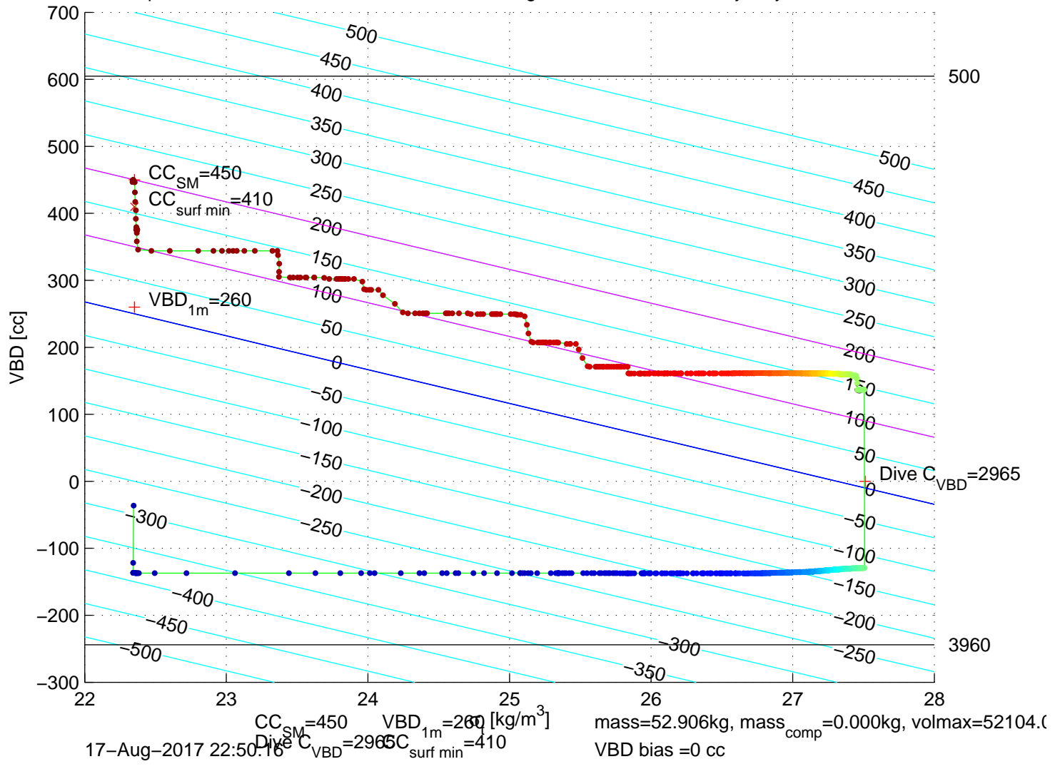
p6100212: SG610 Mission 7 Jul 2017 17-Aug-2017 22:10:52Z – buoyancy contoured
