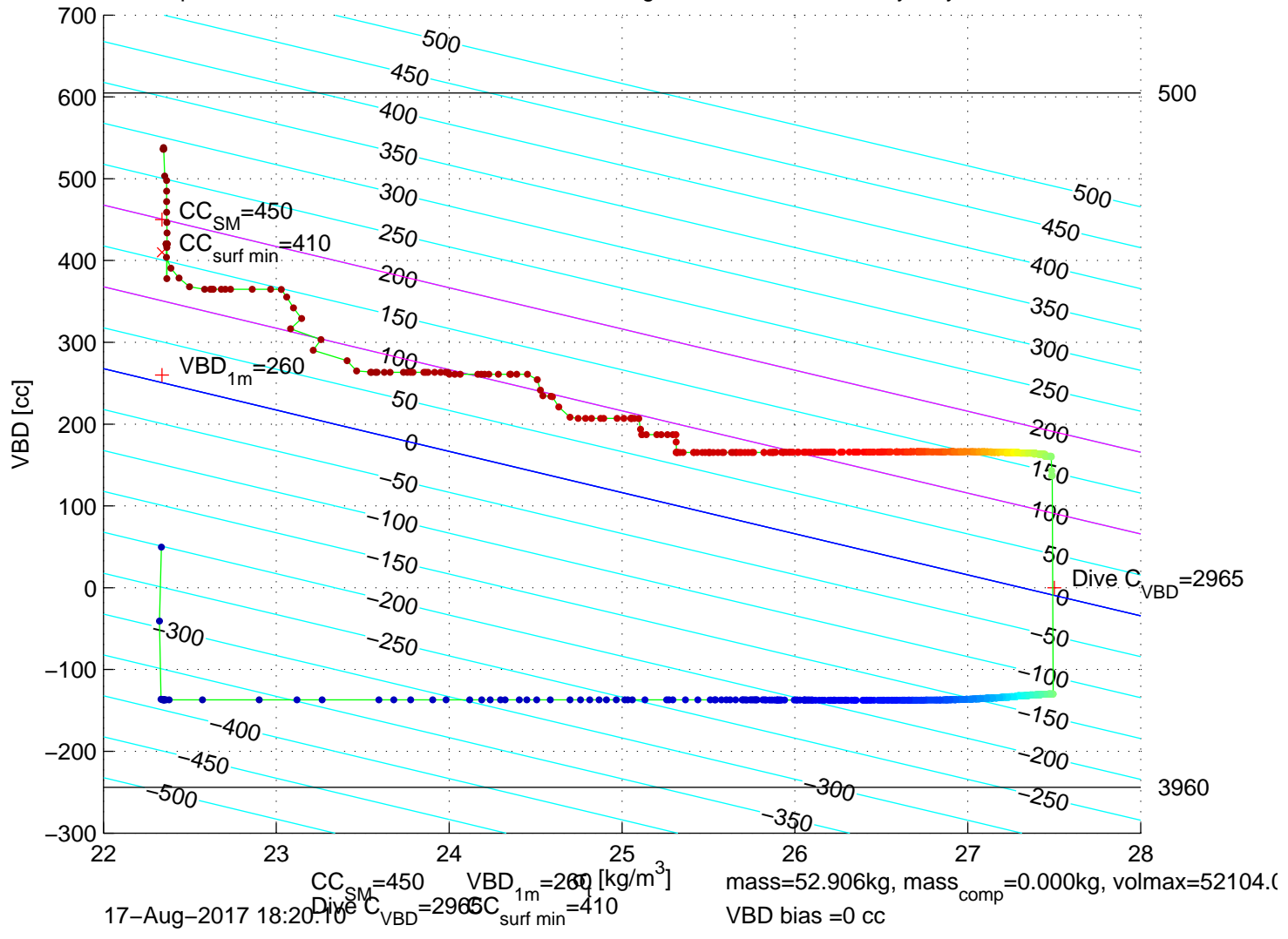
p6100211: SG610 Mission 7 Jul 2017 17-Aug-2017 17:43:44Z – buoyancy contoured
