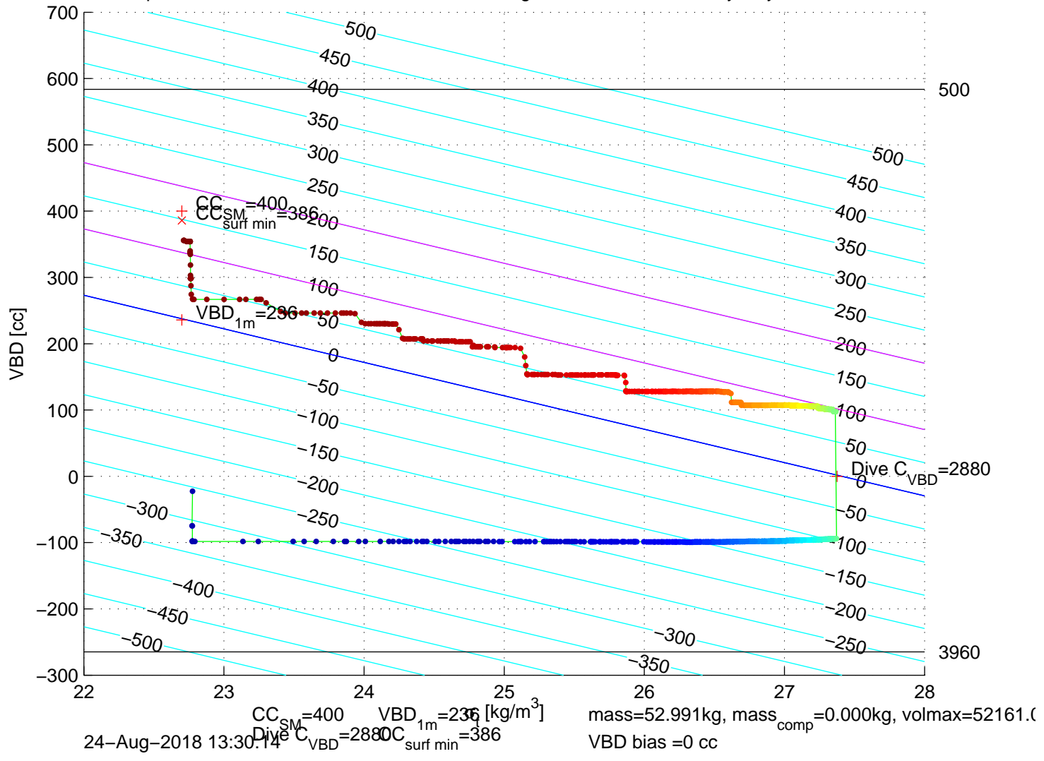
p6100207: SG610 Mission 8 Jul 2018 24-Aug-2018 12:39:29Z – buoyancy contoured
