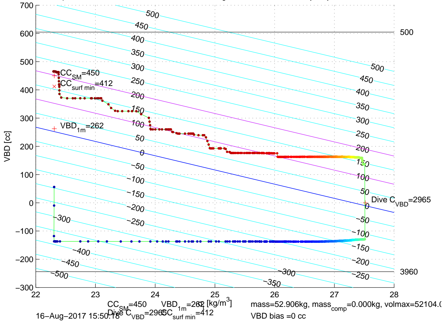
p6100205: SG610 Mission 7 Jul 2017 16–Aug–2017 15:16:41Z – buoyancy contoured
