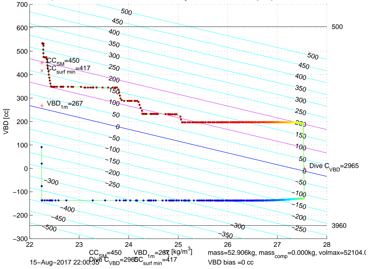
p6100201: SG610 Mission 7 Jul 2017 15–Aug–2017 21:41:04Z – buoyancy contoured
