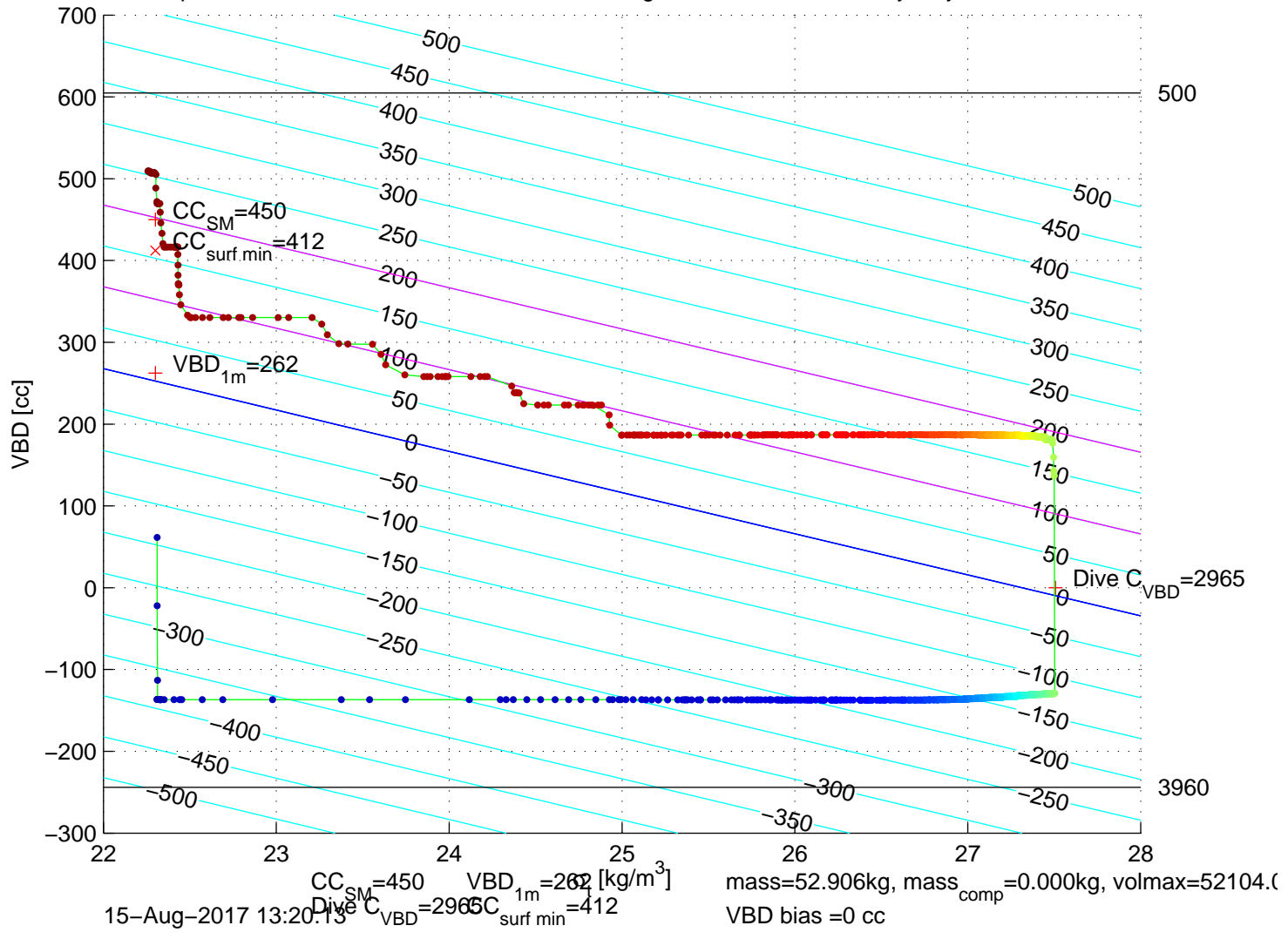
p6100199: SG610 Mission 7 Jul 2017 15–Aug–2017 12:59:01Z – buoyancy contoured
