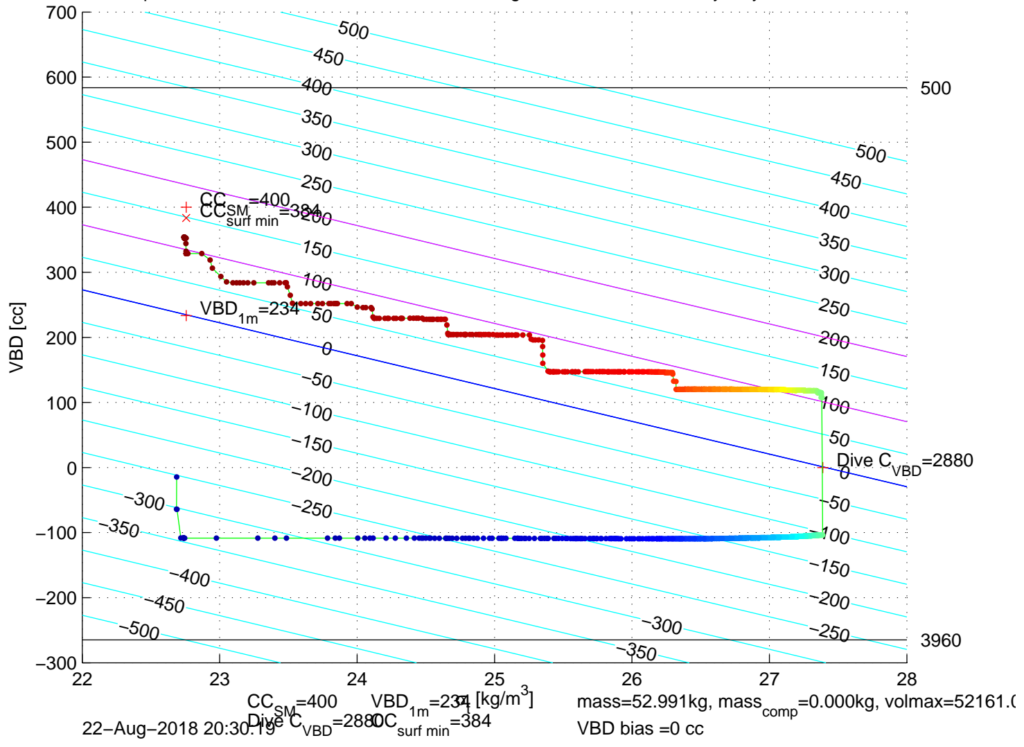
p6100198: SG610 Mission 8 Jul 2018 22-Aug-2018 19:45:05Z – buoyancy contoured
