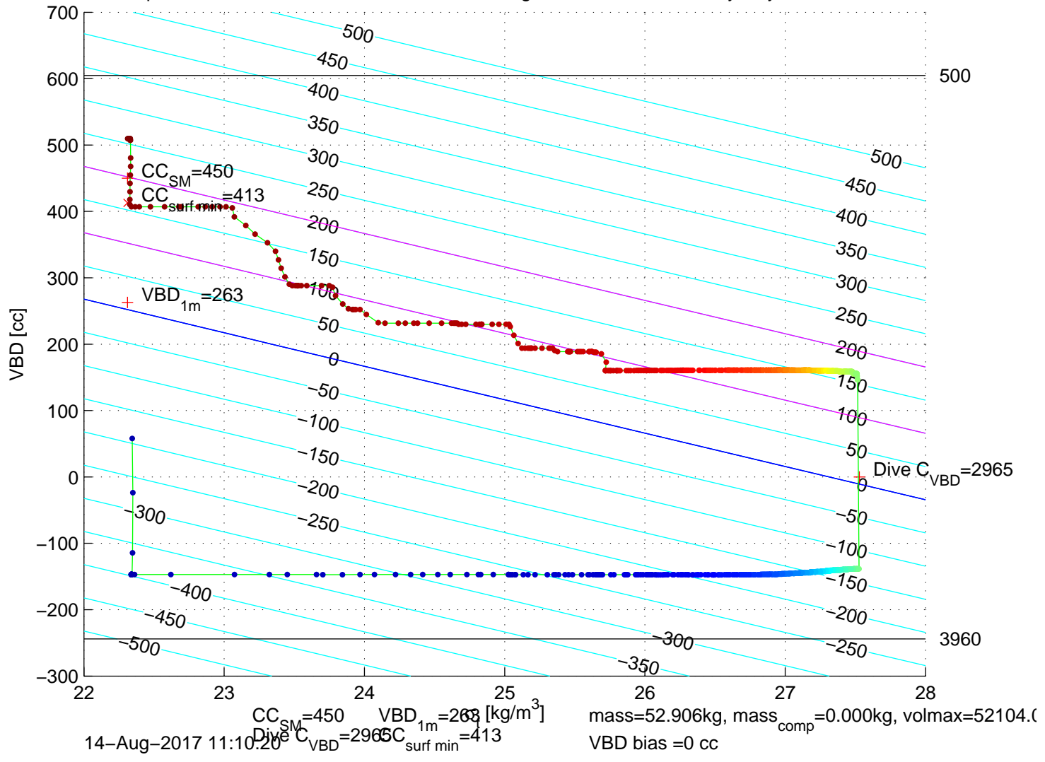
p6100193: SG610 Mission 7 Jul 2017 14-Aug-2017 10:31:01Z – buoyancy contoured
